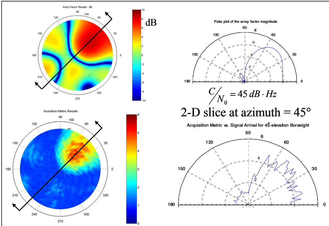
Figure 5. GPS signal correlation metric vs. arrival direction, 7-element CRPA. Left-side shows entire sky (gain and correlation); right-side shows a section at boresight azimuth.
